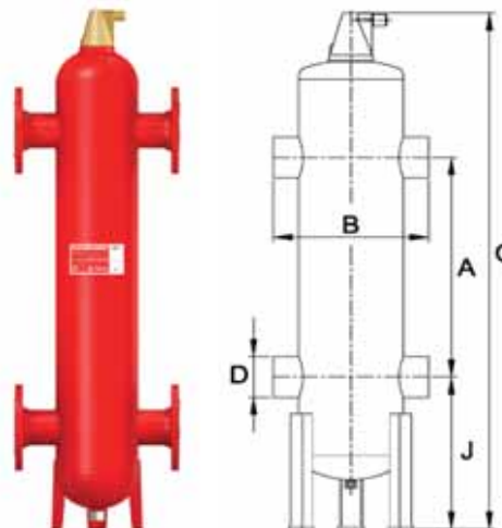
Flexbalance, DN 150–400
